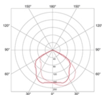
BARI II DOWNLIGHT DLN 230
