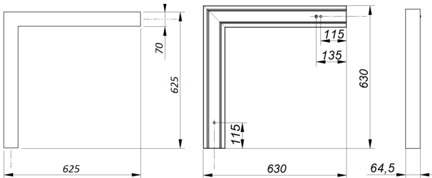
Dimensions of the installation hole
